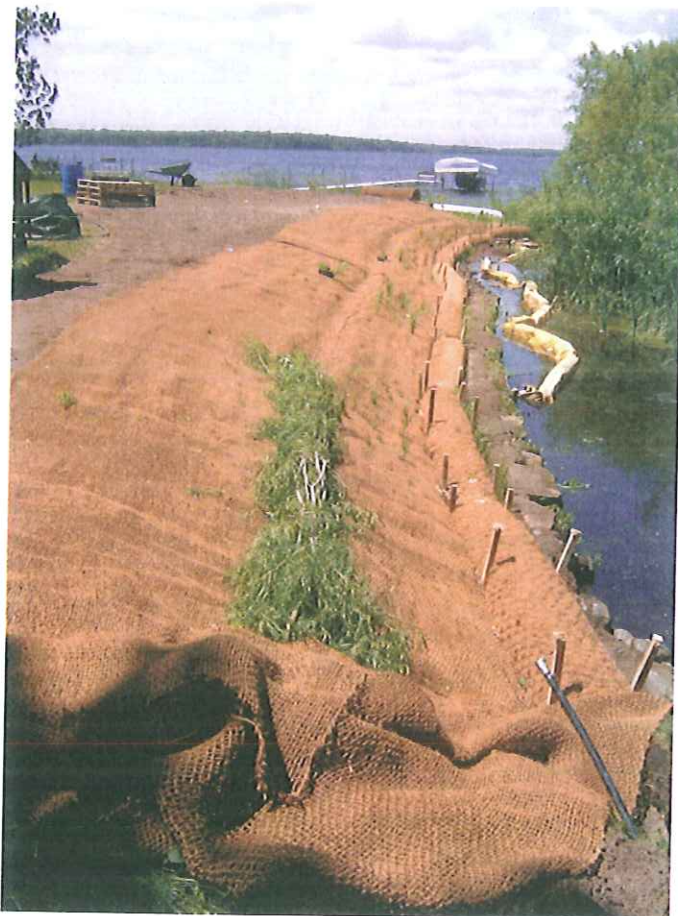
Figure 4.15. Wattles staked in to secure ECBs at their overlap. Notice how the upper blanket overlaps the lower blanket. (Photo: Jane Herbert.)
