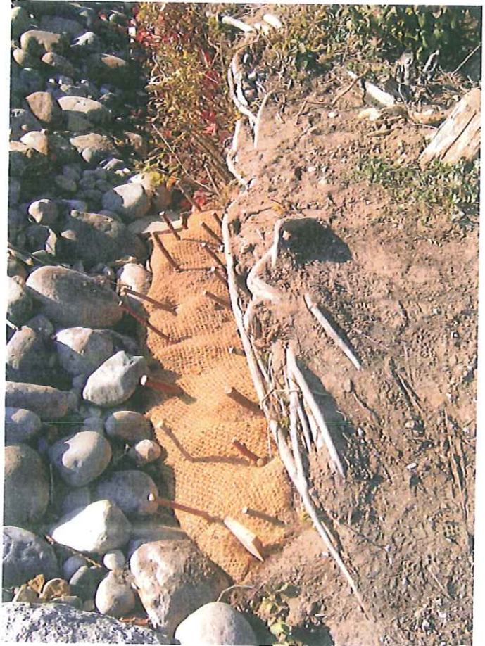
Figure 4.16. Autumn installation of dormant live stakes (foreground) and whips to repair shoreline damaged by an uprooted tree. (Photo: Jane Herbert.)
